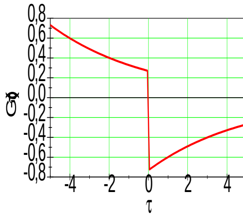
Figure 22-4 \mathcal{G}_0(\mathbf{p}, \tau) for a value of momentum above the Fermi surface.
