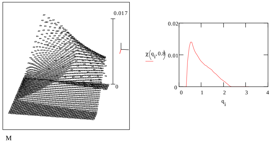
Figure 30-4 Imaginary part of the Lindhard function in d = 3 . Axes like in the d = 1 case.
