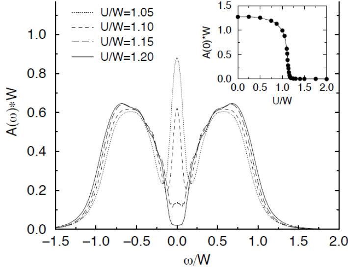
Figure 46-2 decrease for U \gg W ; from Ref. [78] in Vollhardt in Mancini.
