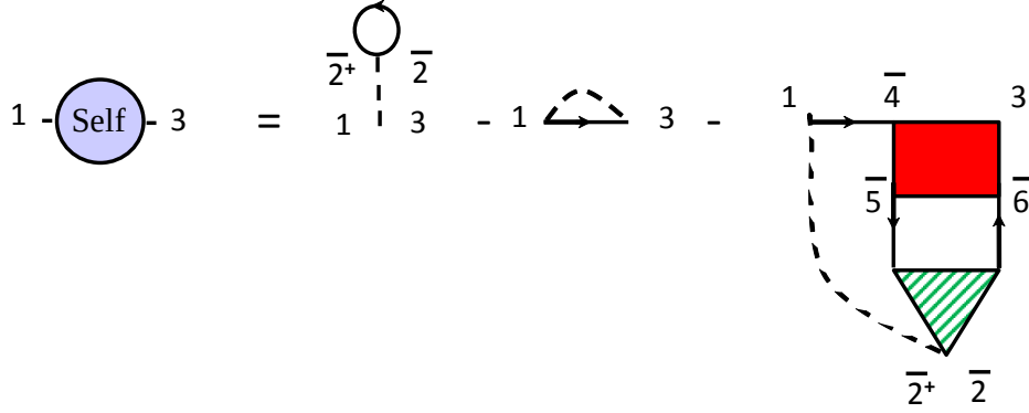
Figure 27-2 Diagrams for the self-energy. The dashed line represent the interaction. The first two terms are, respectively, the Hartree and the Fock contributions. The textured square appearing in the previous figure for the four-point function has been squeezed to a triangle to illustrate the fact that two of the indices (coordinates) are identical.
