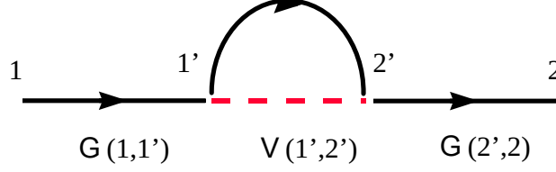
Figure 29-2 A typical contraction for the first-order expansion of the Green's function. The Fock term.
