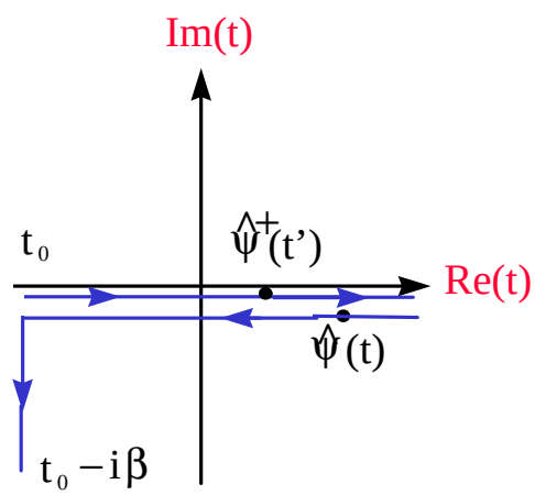
Figure 21-2 Keldysh-Schwinger contour.
