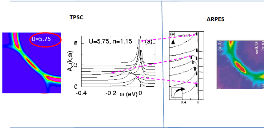
Figure 49-2 On the left, results of TPSC calculations [?, ?] at optimal doping, x = 0.15 , corresponding to filling 1.15, for t = 350 meV, t' = -0.175t , t_j = 0.05t , U = 5.75t , T = 1/20 . The left-most panel is the magnitude of the spectral weight times a Fermi function, A(\mathbf{k}, \omega) f(\omega) at \omega = 0 , so-called momentum-distribution curve (MDC). Red (dark black) indicates larger value and purple (light grey) smaller value. The next panel is A(\mathbf{k}, \omega) f(\omega) for a set of fixed \mathbf{k} values along the Fermi surface. These are so-called energy-dispersion curves (EDC). The two panels to the right are the corresponding experimental results [?] for \text{Nd}_{2-x}\text{Ce}_x\text{CuO}_4 . Dotted arrows show the correspondence between TPSC and experiment.
