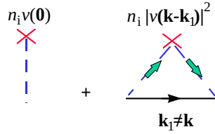
Figure 15-2 Second-order irreducible self-energy in the impurity averaging technique.
