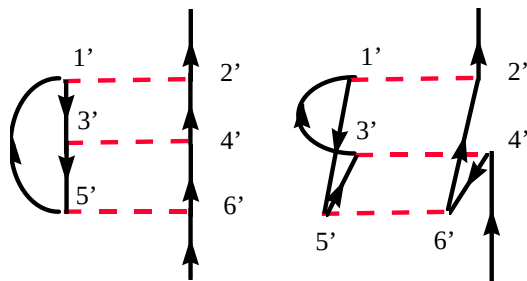
Figure 29-4 Two topologically equivalent diagrams of order 3.
