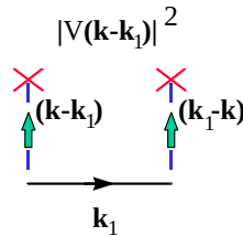
Figure 13-7 Second order irreducible self-energy (before impurity averaging). Note that \mathbf{k}_1 \neq \mathbf{k} . That is why this diagram is irreducible.
