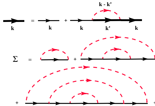
Figure 33-2 Hartree-Fock as a self-consistent approximation for the Green's function. This self-consistent approximation is equivalent to a self-energy that sums all the rainbow diagrams illustrated on the bottom part of the figure. The thick line is the full Green's function.
