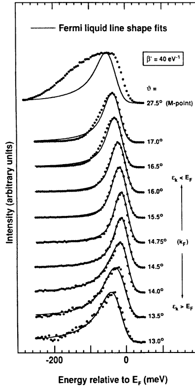
Figure 23-1 ARPES spectrum of 1 - T - TiTe_2 , after R. Claessen, R.O. Anderson, J.W. Allen, C.G. Olson, C. Janowitz, W.P. Ellis, S. Harm, M. Kalning, R. Mancke, and M. Skibowski, Phys. Rev. Lett 69 , 808 (1992).
