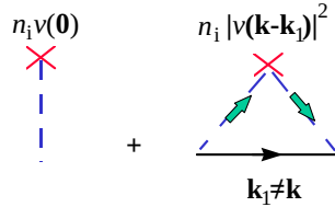
Figure 15-4 Second-order irreducible self-energy in the impurity averaging technique.
