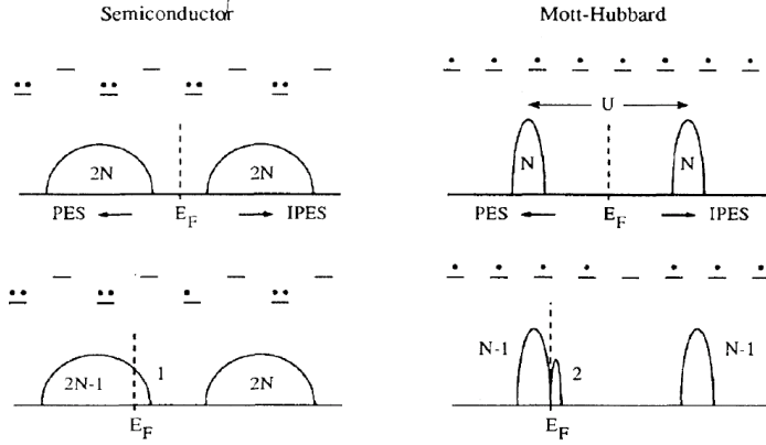
Figure 46-2 decrease for U \gg W ; from Ref. [78] in Vollhardt in Mancini.
