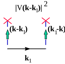
Figure 13-6 Second order irreducible self-energy (before impurity averaging). Note that \mathbf{k}_1 \neq \mathbf{k} . That is why this diagram is irreducible.
