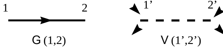
Figure 29-1 Basic building blocks of Feynman diagrams for the electron gas.
