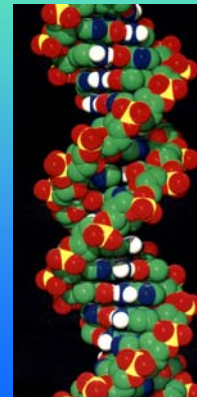
DNA molecule
