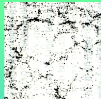
Zeldovich distribution
