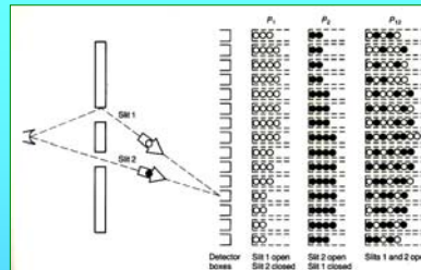
Pattern of arrivals of classical particles when one or other of the slits is open, & when both are open.
