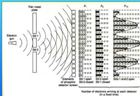
Pattern of arrivals of electrons with the same combination of slits open or closed.
