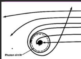
Below: light paths near a black hole
