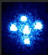
"Einstein's cross"
