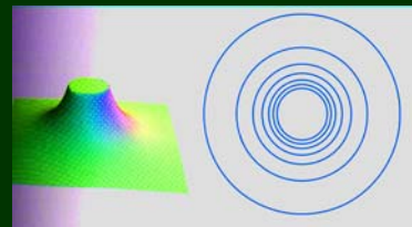
Electrostatic potential from +ve charge
