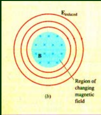
Electric field around changing B-field
