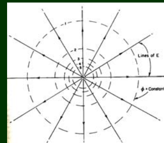
Field lines from +ve charge
